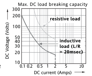
Graph 2 DC ratings
